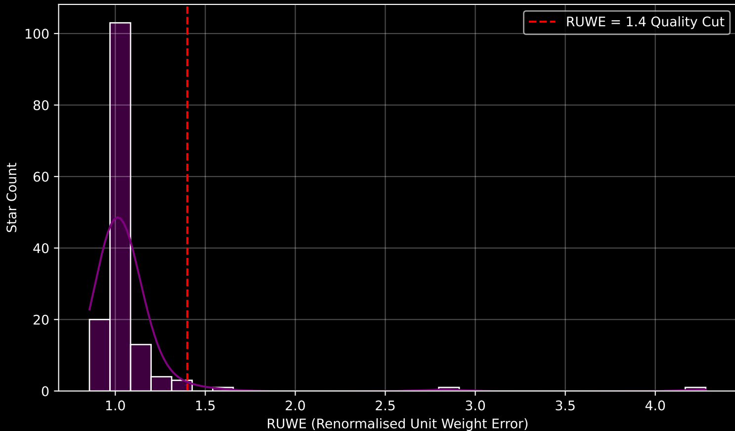
GAPOGEE DR17 Field [Per_E] RUWE Distribution (n= 146)
