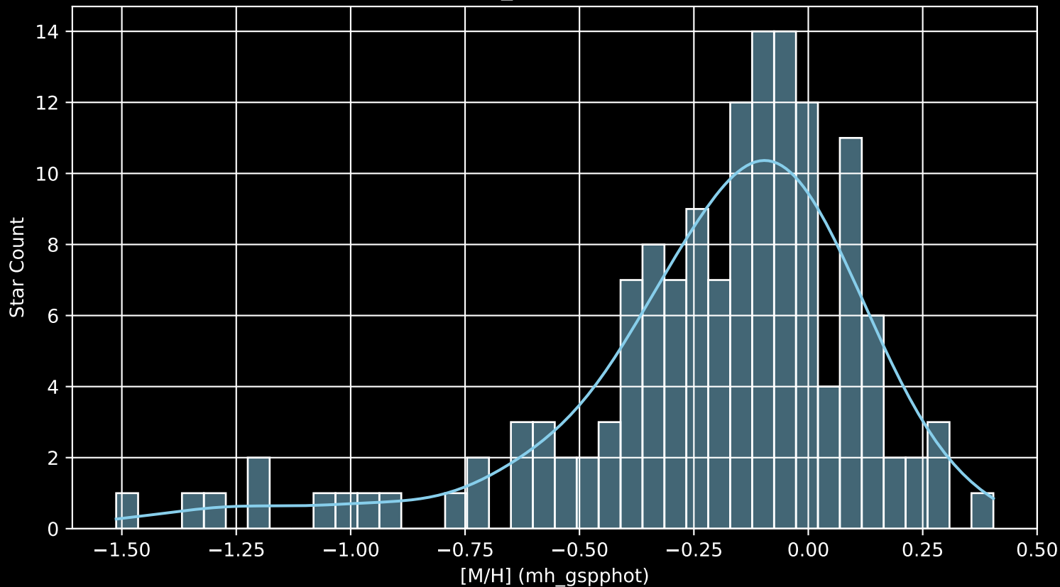
APOGEE DR17 Field: [Per_E [M/H] (mh_gspphot) (n= 144)
