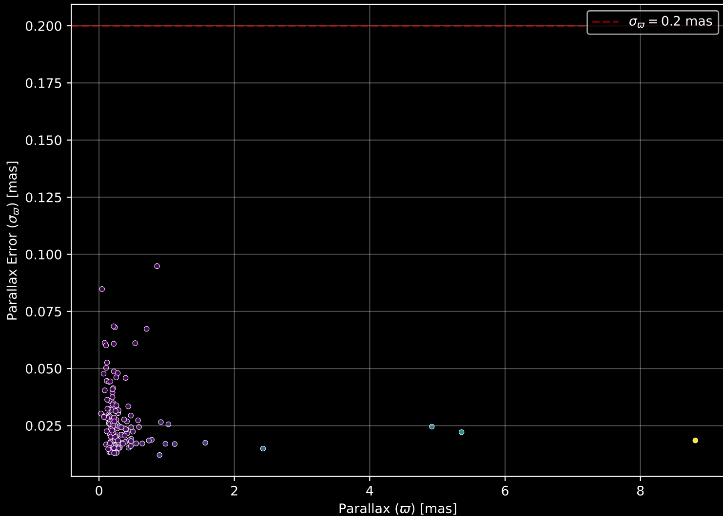
APOGEE DR17 Field: [Per_E] Parallax Quality (n= 147)
