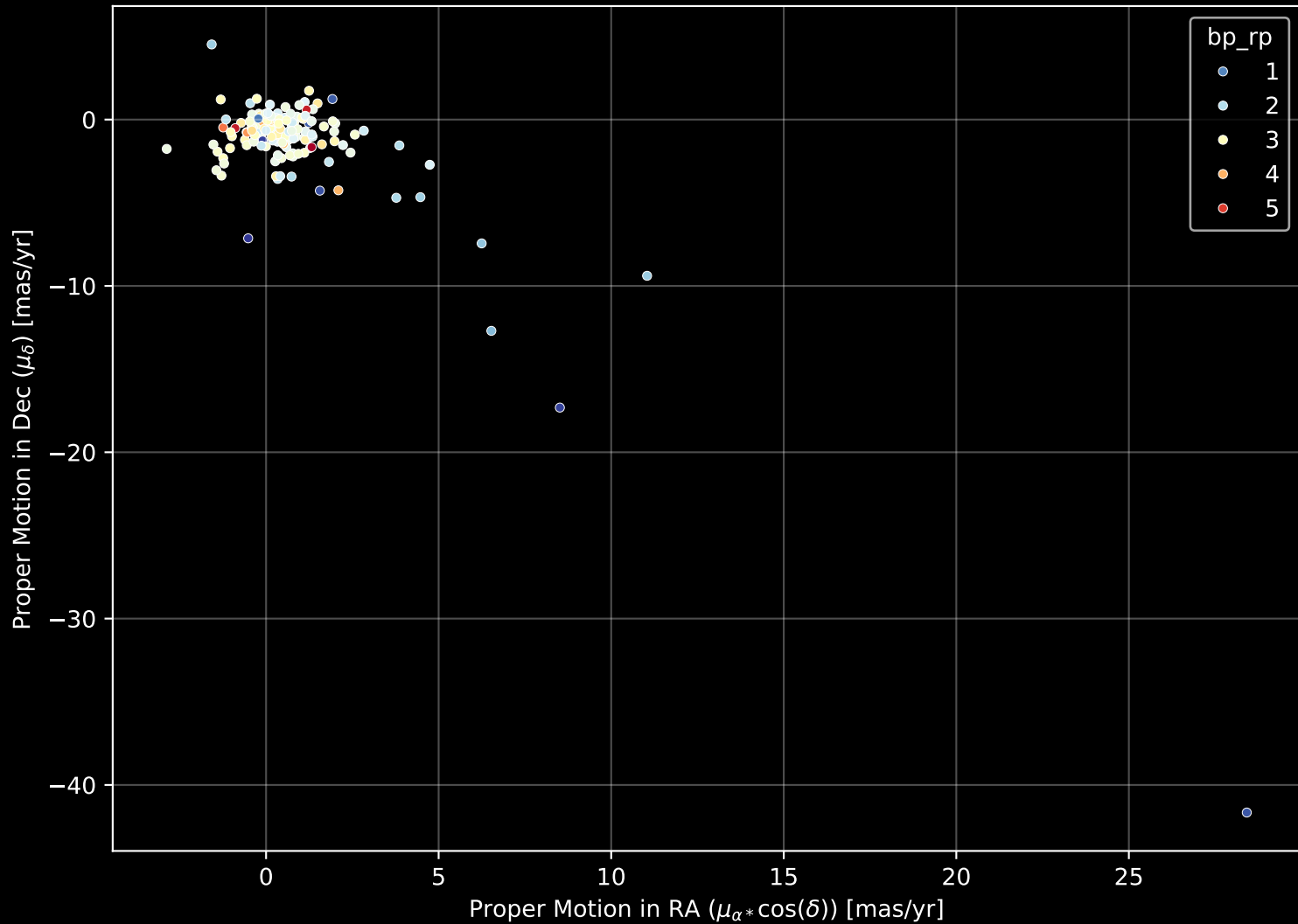
APOGEE DR17 Field: [Per_E] Proper Motion Diagram (n= 147)
