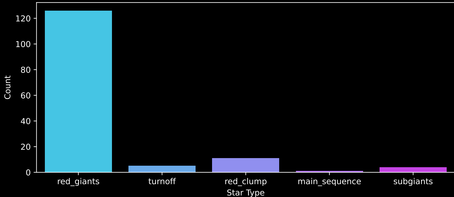
APOGEE DR17 Field: [Per_E] Count plot of Star Type
